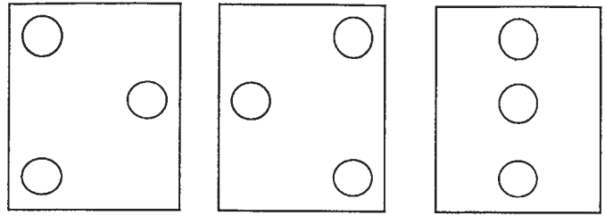
FIG. 3 Impact Locations for Small Missile Test (Each Type of Infill)
