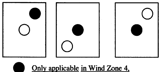
FIG. 1 Impact Location for Large Missile Test (Each Type of Infill)
